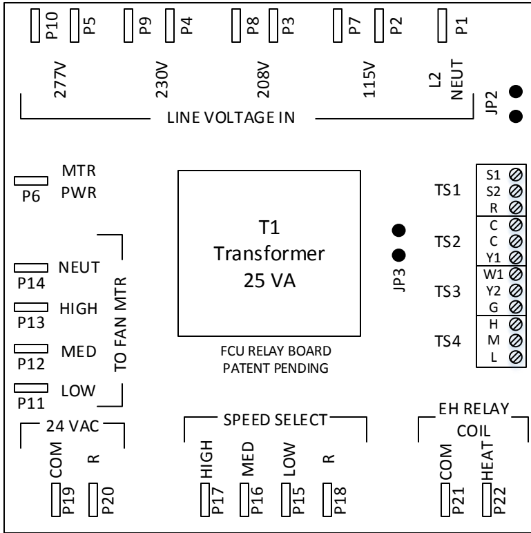
Fan Coil Relay Board - FCRB
